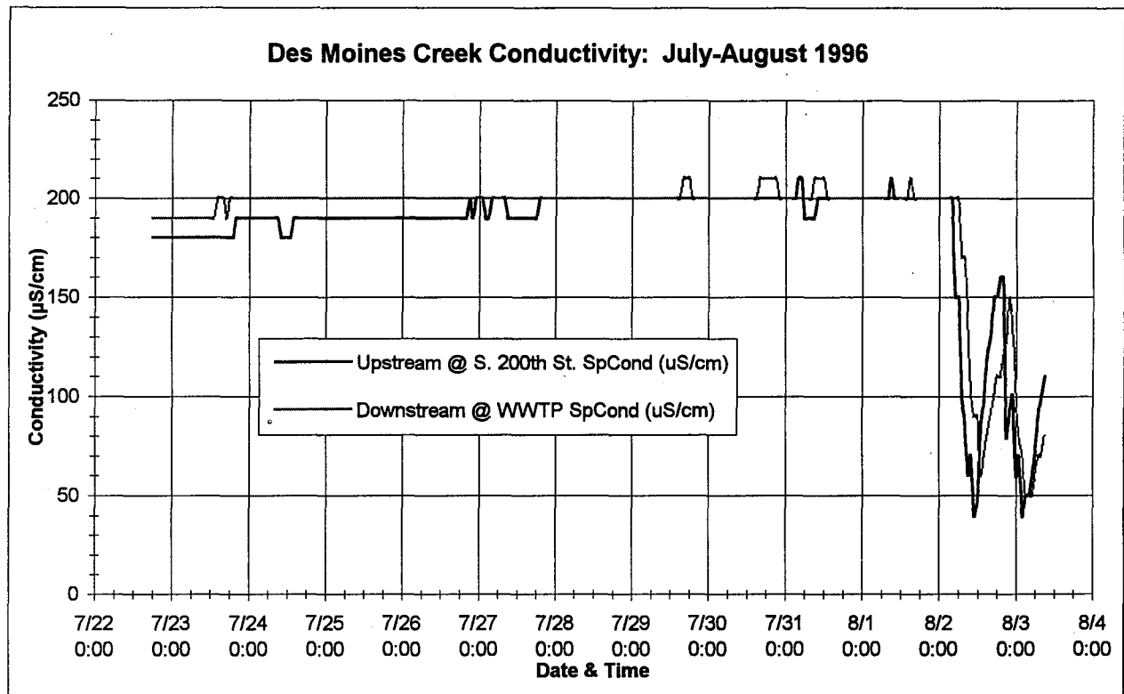
Figure B.5 (continued). Des Moines Creek conductivity at Upstream (S. 200th St.) and Downstream (WWTP) baseflow monitoring stations.
