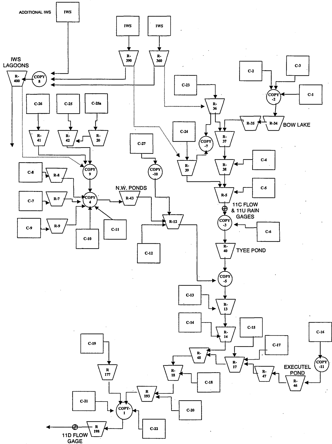
Figure A.2 Des Moines Creek Watershed Model Schematic
