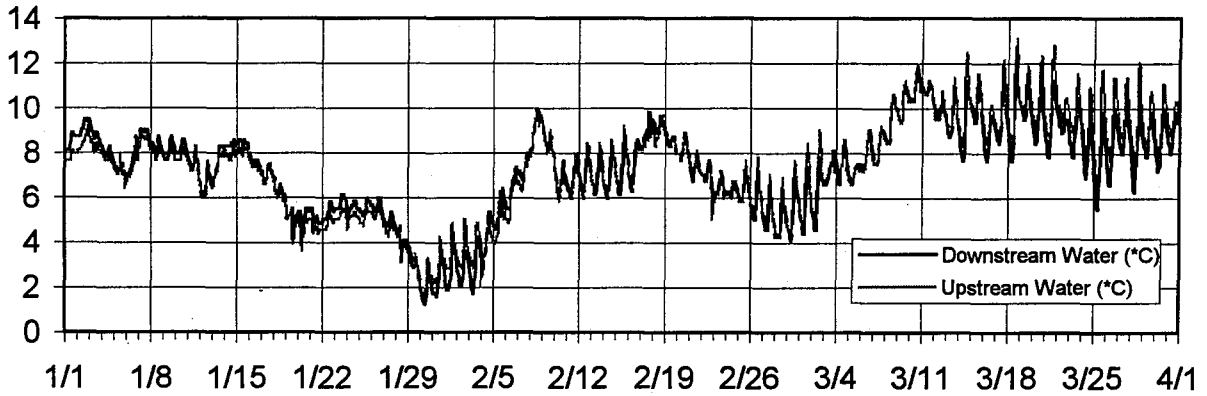
Des Moines Creek - Water Temperature January-March 1996
