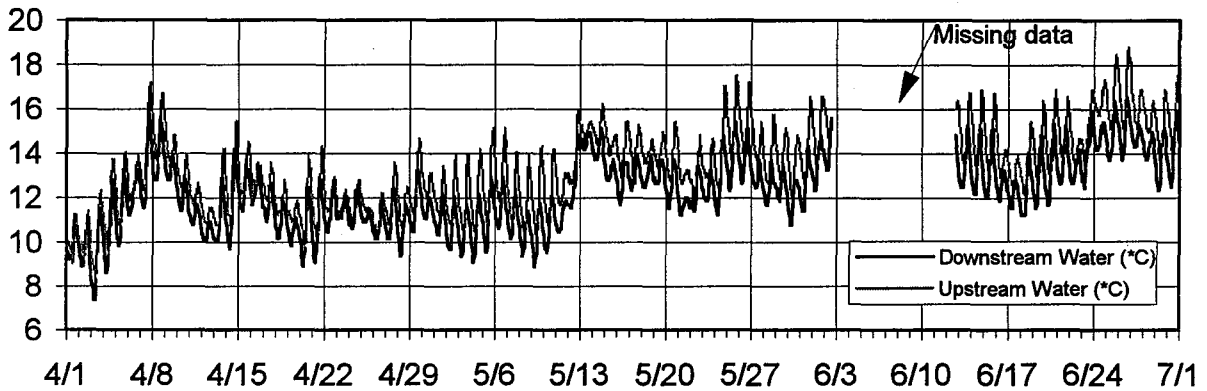
Des Moines Creek - Water Temperature April-June 1996
